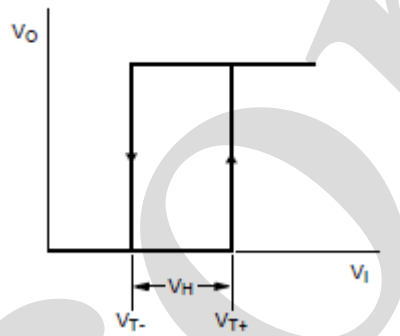
Figure 6. Transfer characteristic
